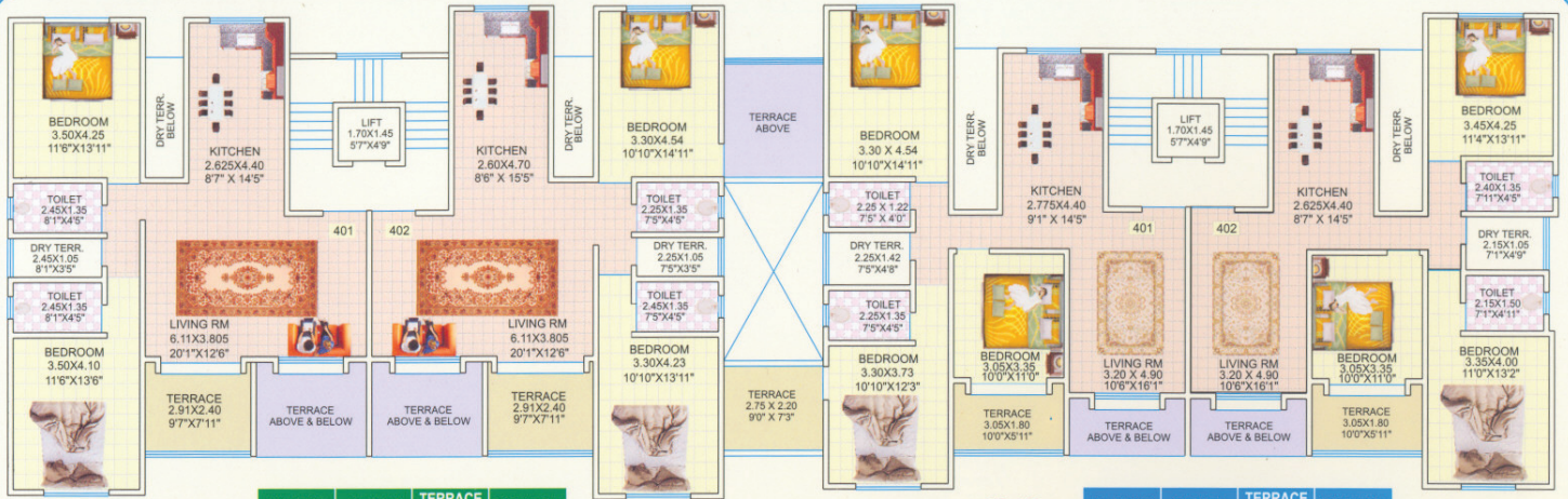
4th Floor 'C' wing
