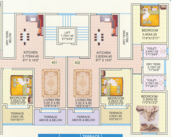
4th Floor 'B' wing
