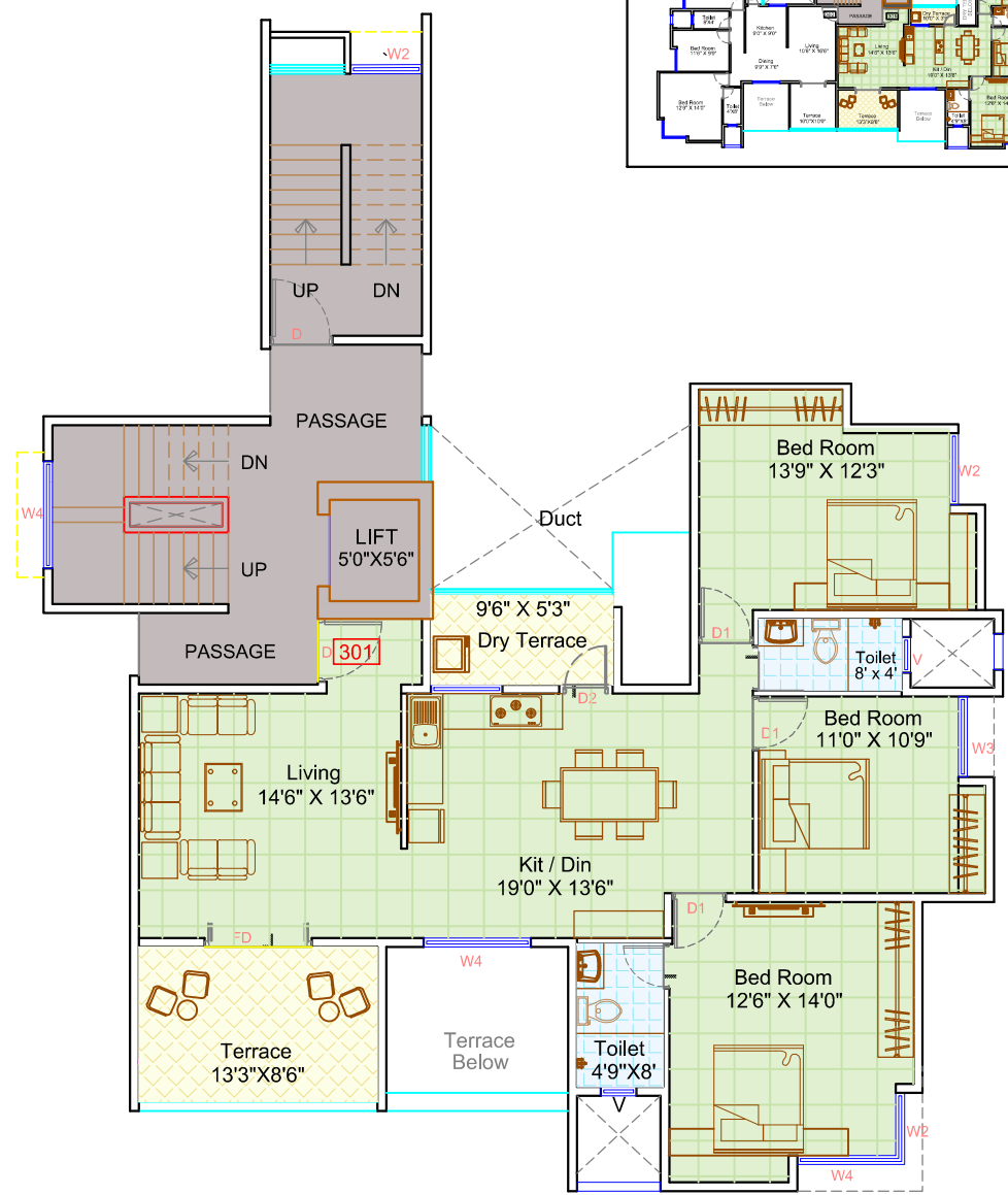
THIRD FLOOR PLAN FLAT NO - 301
